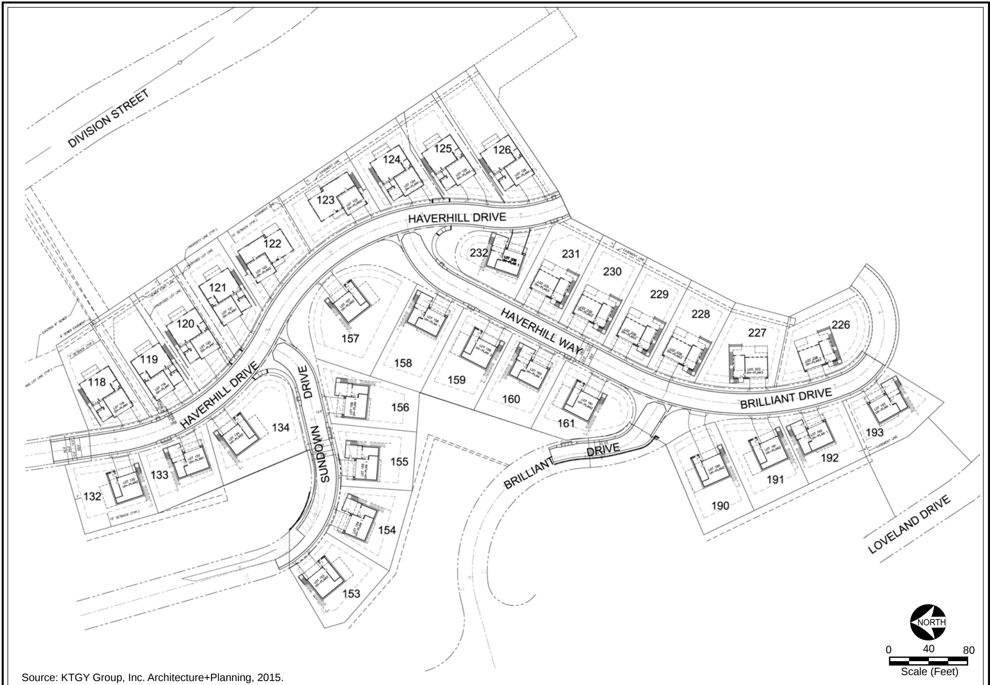
Figure 2-5 Site Plan
